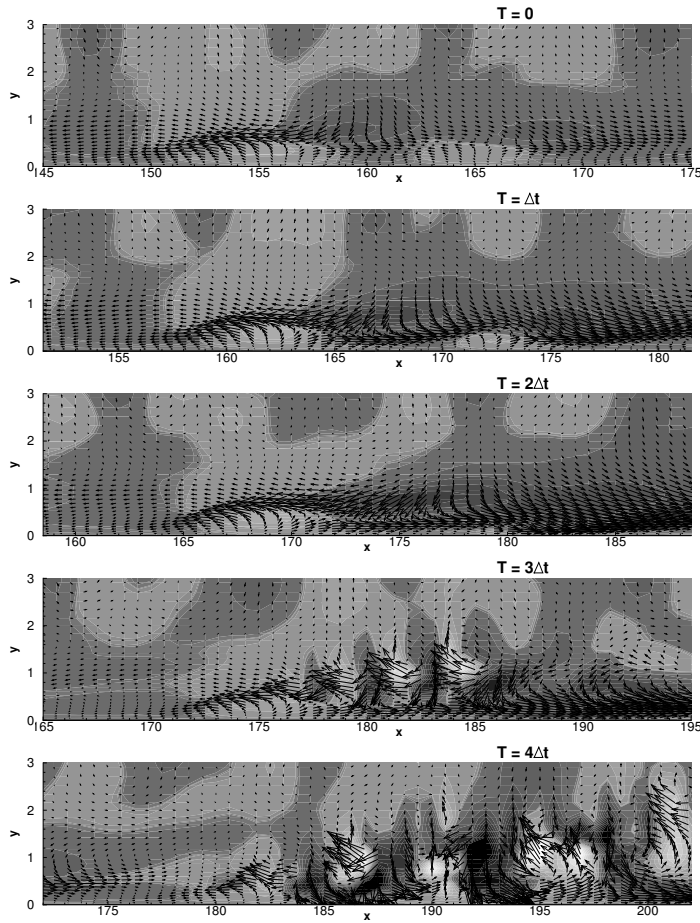
Figure 3.14: Instantaneous v' contours for Tu = 2\% and A = 0.5\% in the x - y plane passing through the incipient turbulent spot in figure 3.13(b) at representative times. Contours are plotted for -0.1 \leq v' \leq 0.1 . In-plane perturbation velocity vectors are shown. The frames are separated by \Delta t = 0.0625\tau where \tau represents one flow-through time.
