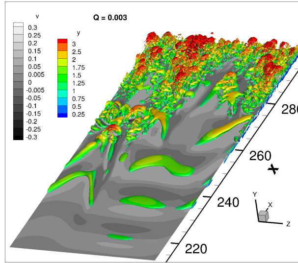
Figure 4.19: Formation and breakdown of \Lambda vortices depicted by isosurfaces of Q -criteria. The isosurfaces of Q = 0.003 are color contoured by distance from the wall. -0.3 \leq v' \leq 0.3 contours are also shown in a horizontal plane at a wall normal height y = \delta_0 .
