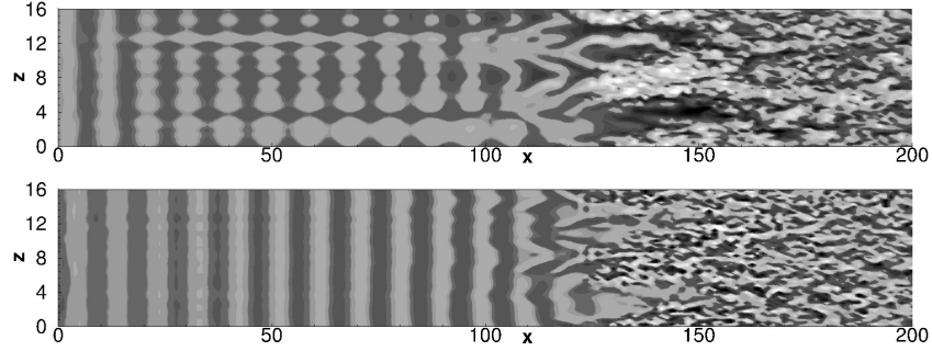
Figure 3.4: Instantaneous u' (top) and v' (bottom) fluctuation velocity contours for Tu = 1\% and A = 1\% in the horizontal x-z plane at y = \delta_0/3 . Contours are plotted for -0.3 \leq u' \leq 0.3 and -0.1 \leq v' \leq 0.1 .
