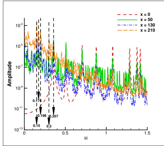
Figure 4.14: Frequency spectra of the u' component at specified streamwise locations for the case tu0011.
